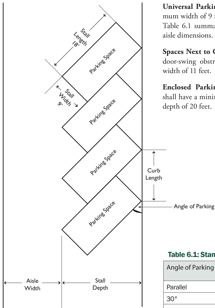
Figure 6-1: Parking
